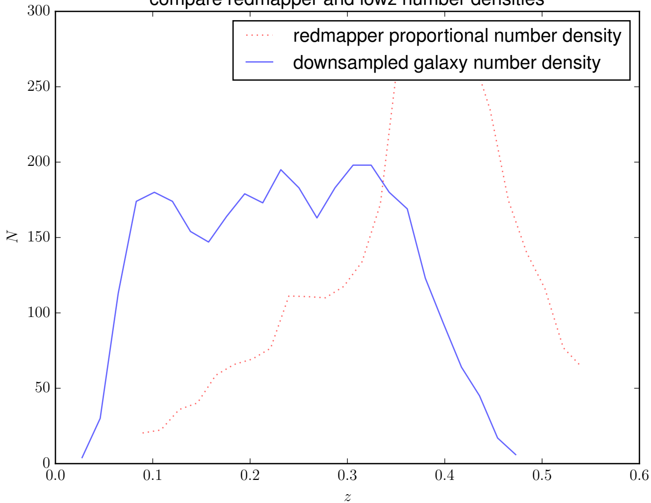
compare redmapper and lowz number densities
