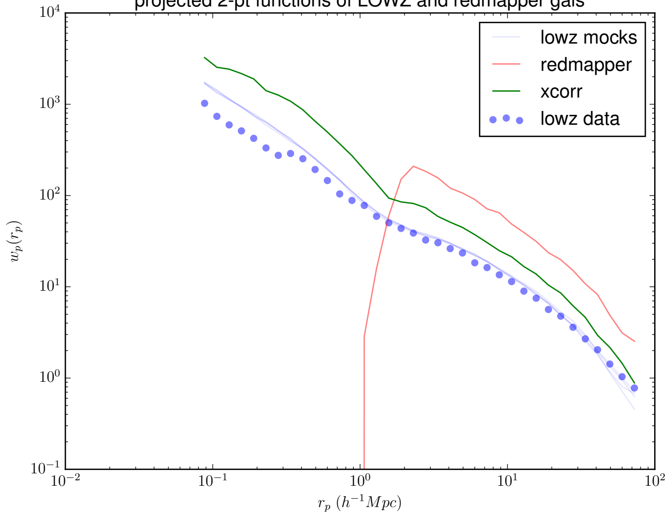
projected 2-pt functions of LOWZ and redmapper gals
