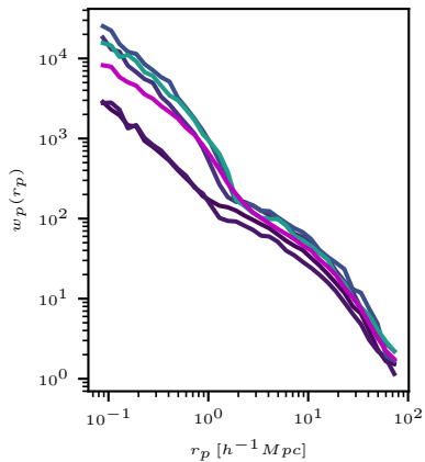
sim gal-cluster xcorr
