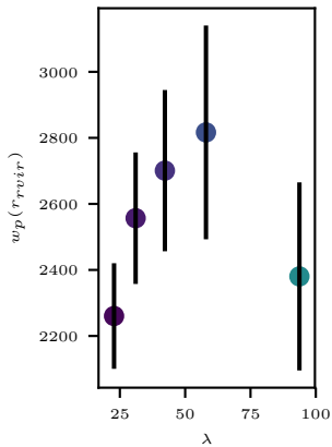
sim gal density v cluster richness
