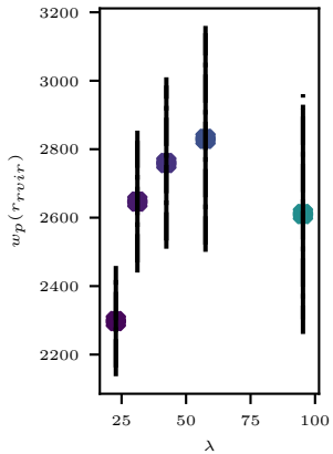
sim gal density v cluster richness
