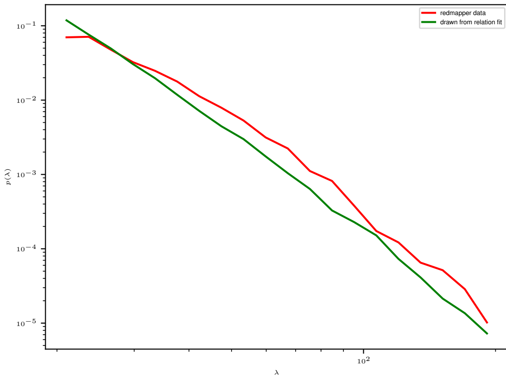
comparison of modeled richness distribution with data
