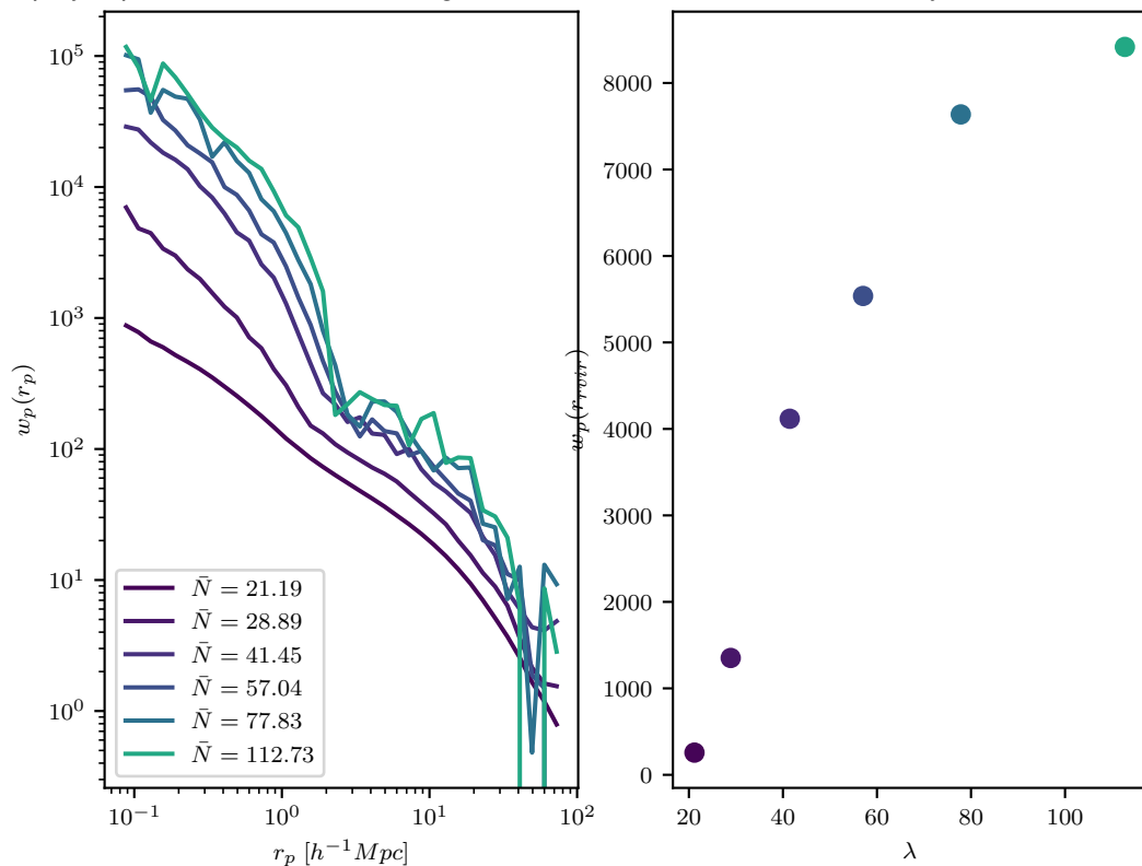
proj. 2-pt xcorr func of simulated gals and clusters mean cluster no. density vs. mean richness
