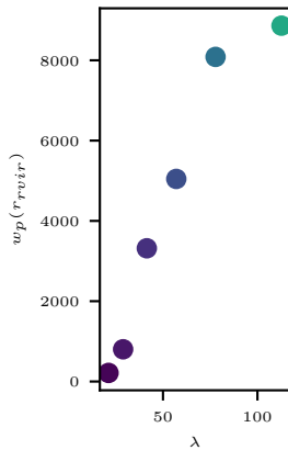
sim gal density v cluster richness
