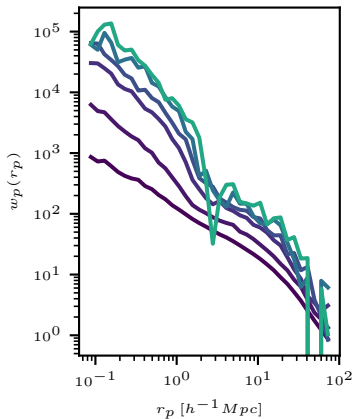
sim gal-cluster xcorr
