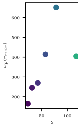
sim gal density v cluster richness
