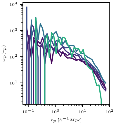
sim gal-cluster xcorr
