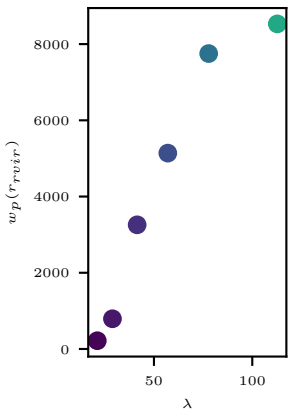
sim gal density v cluster richness
