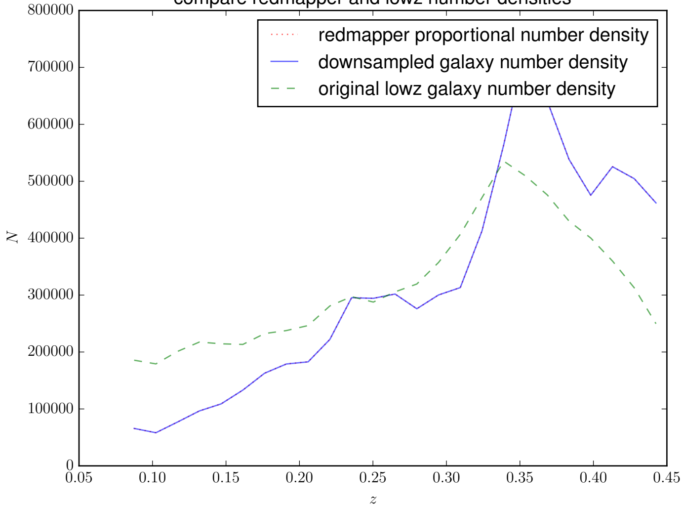
compare redmapper and lowz number densities
