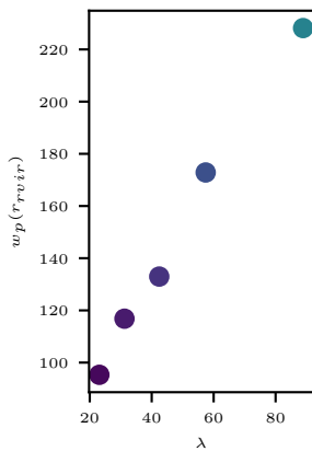
sim gal density v cluster richness
