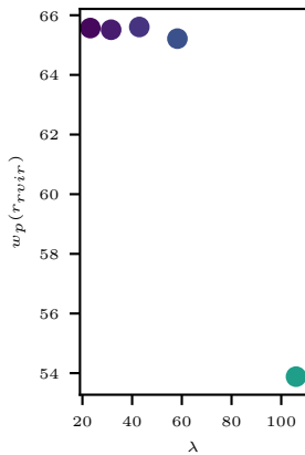
sim gal density v cluster richness
