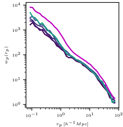
sim gal-cluster xcorr
