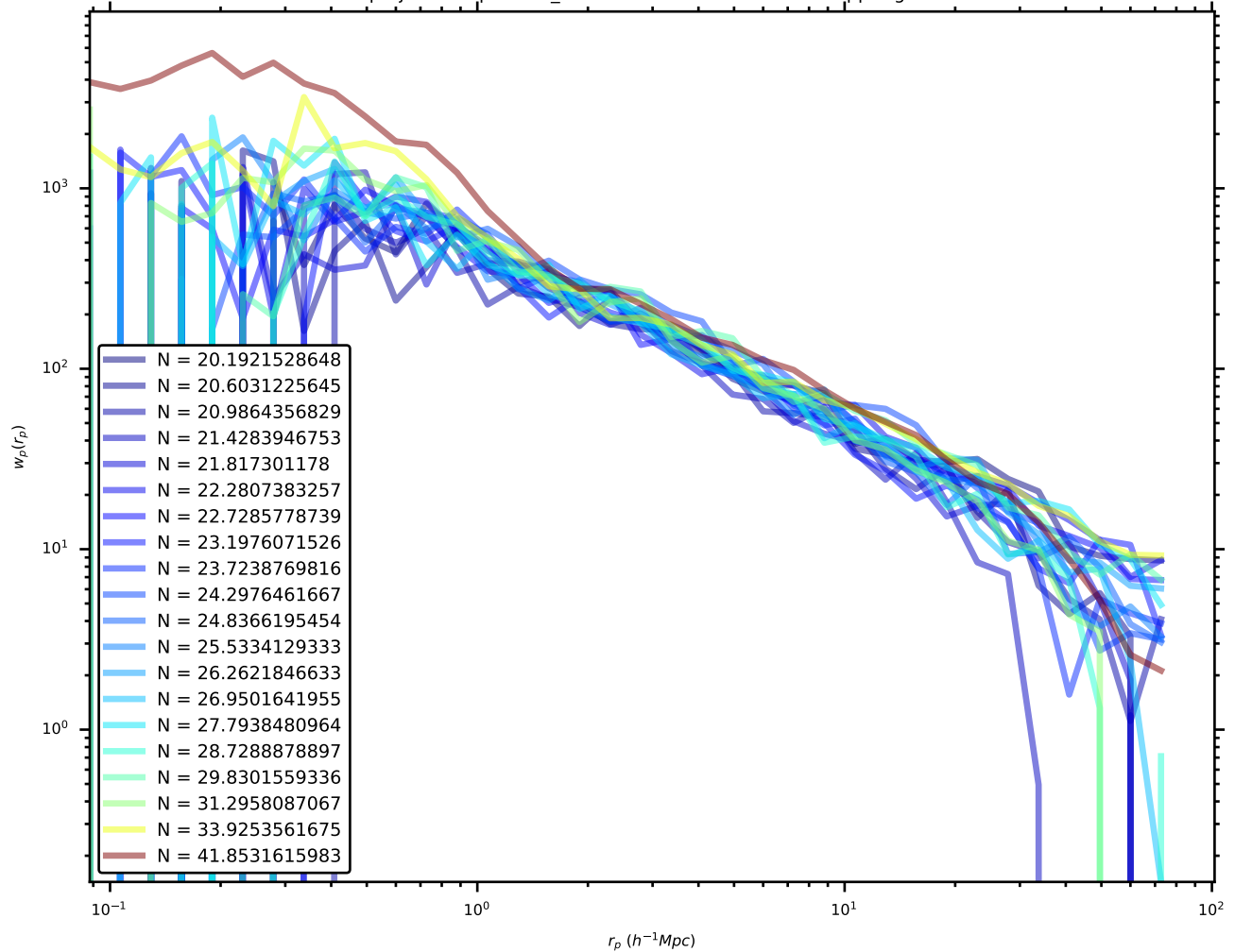
projected 2-pt cross_correlation of LOWZ and redmapper gals
