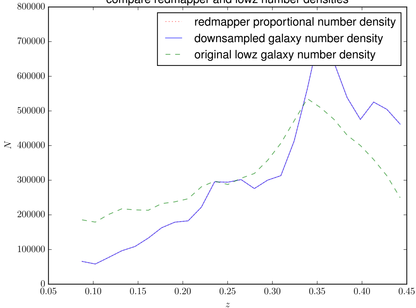
compare redmapper and lowz number densities
