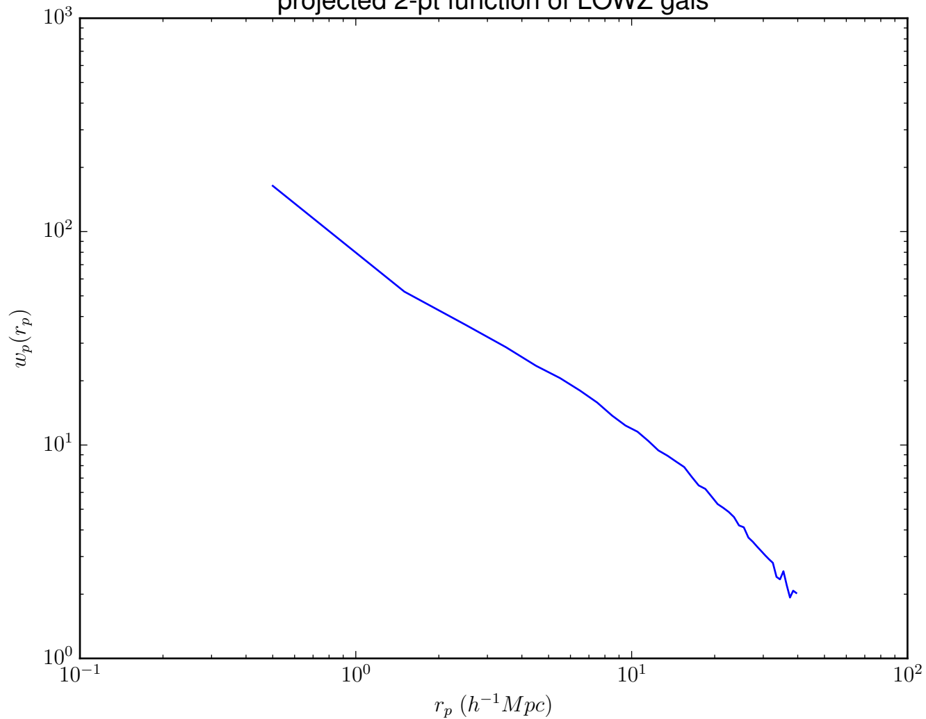
projected 2-pt function of LOWZ gals
