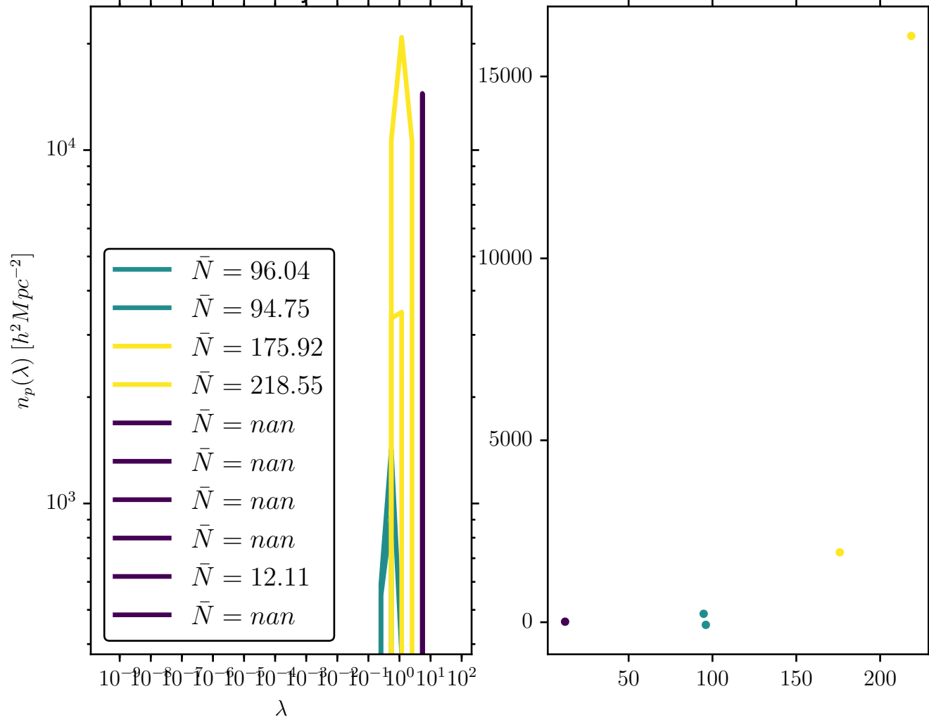
mean cluster no. density vs. mean richness
